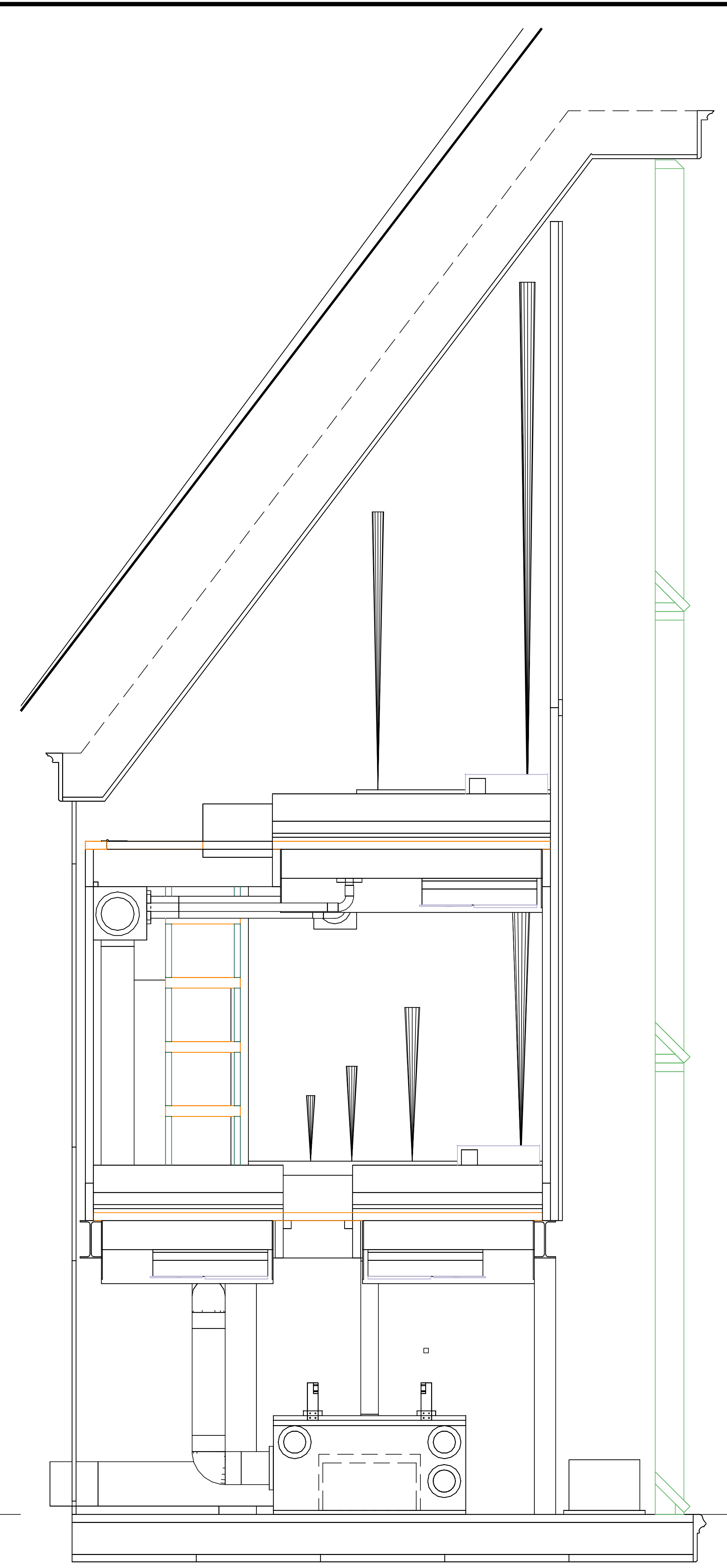
C SWELL (chests) FRONT SECTION VIEW (SCALE: 1" = 1')
