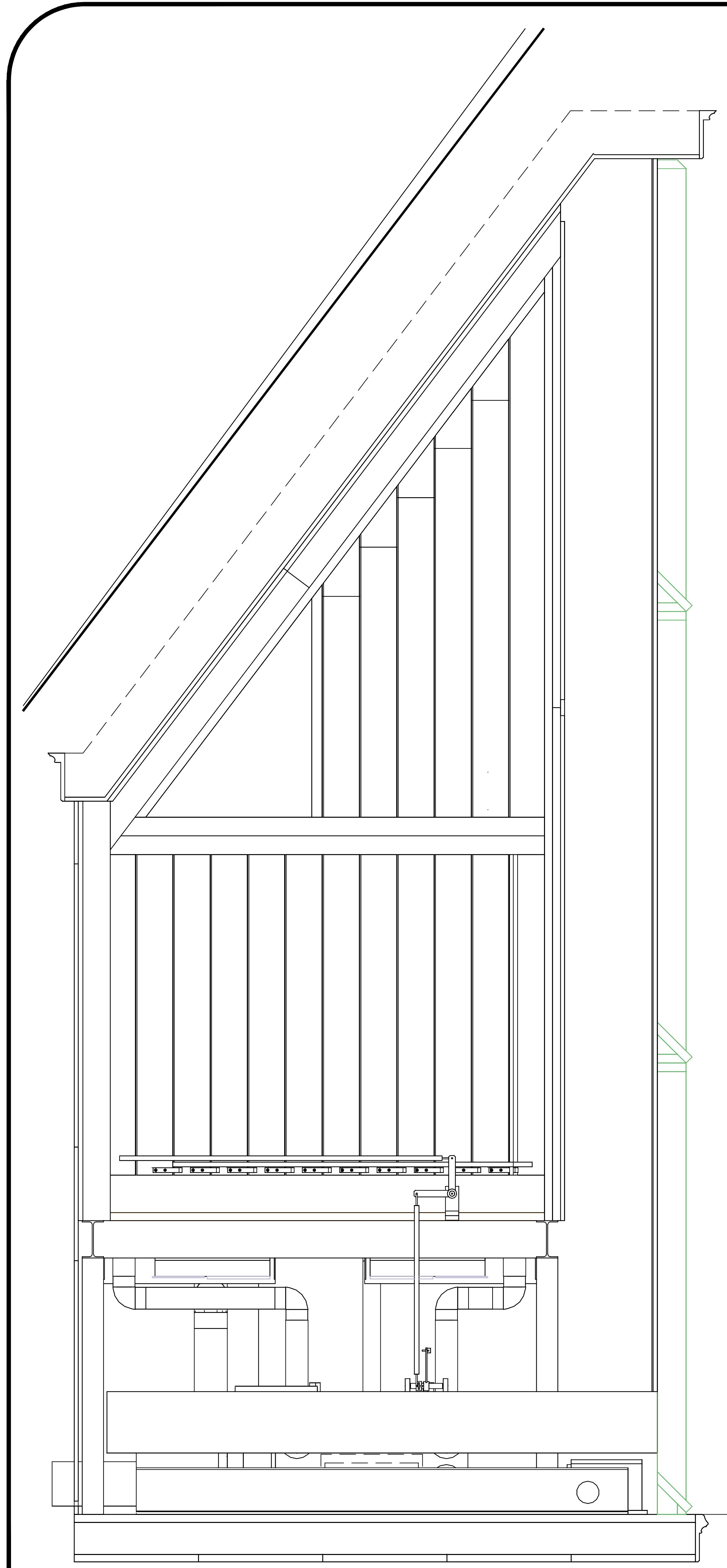
C SWELL (shades) FRONT SECTION VIEW (SCALE: 1" = 1')
